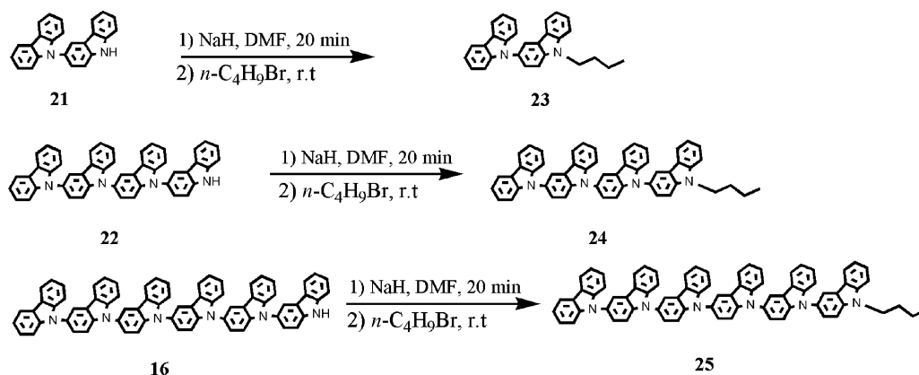
Scheme 4. Synthesis of reference compounds 23–25 .
