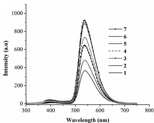
Figure 2. Emission spectra of 1–7 at 1 \mu M in CHCl 3 ( \lambda_{ex} = 295 nm).
