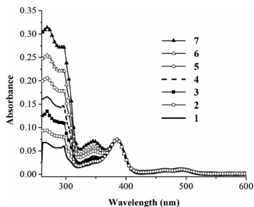
Figure 1. UV/Vis absorption spectra (normalized at the Soret bands) of 1–7 in CHCl 3 .
