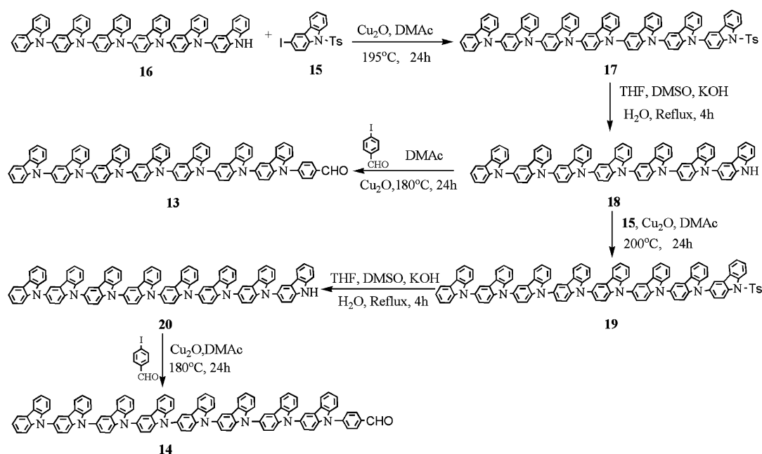
Scheme 2. Synthesis of the precursors of aldehydes 13 and 14 .
