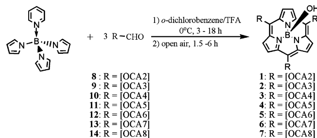
Scheme 3. Synthesis of T(OCA n )SubPs 1–7 .
