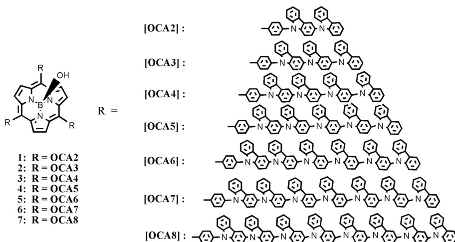
Scheme 1. Molecular structures of T(OCA n )SubPs 1–7.
